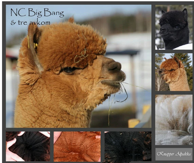
Big Bang
