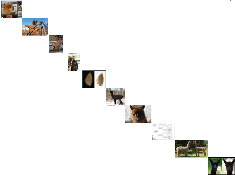
Big Bang
